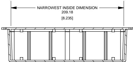
SECTION C-C
